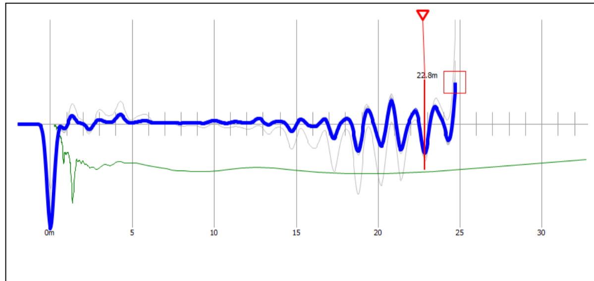
Reflectogram P-152
