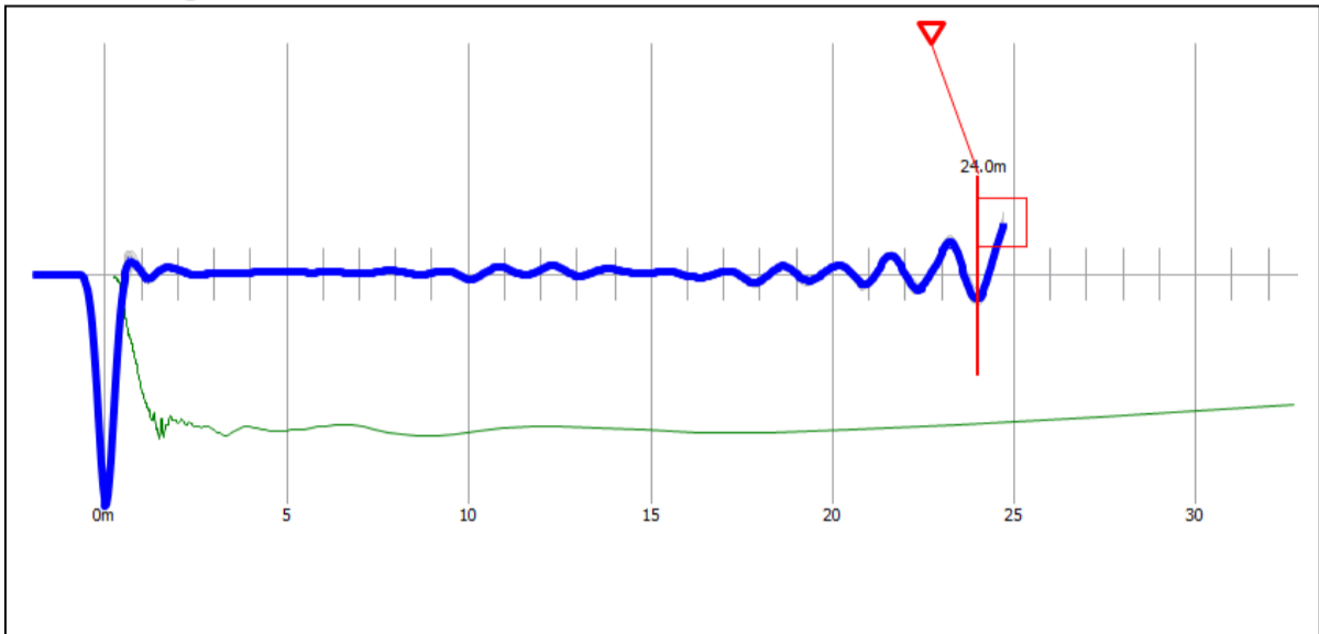
Reflectogram P-265
