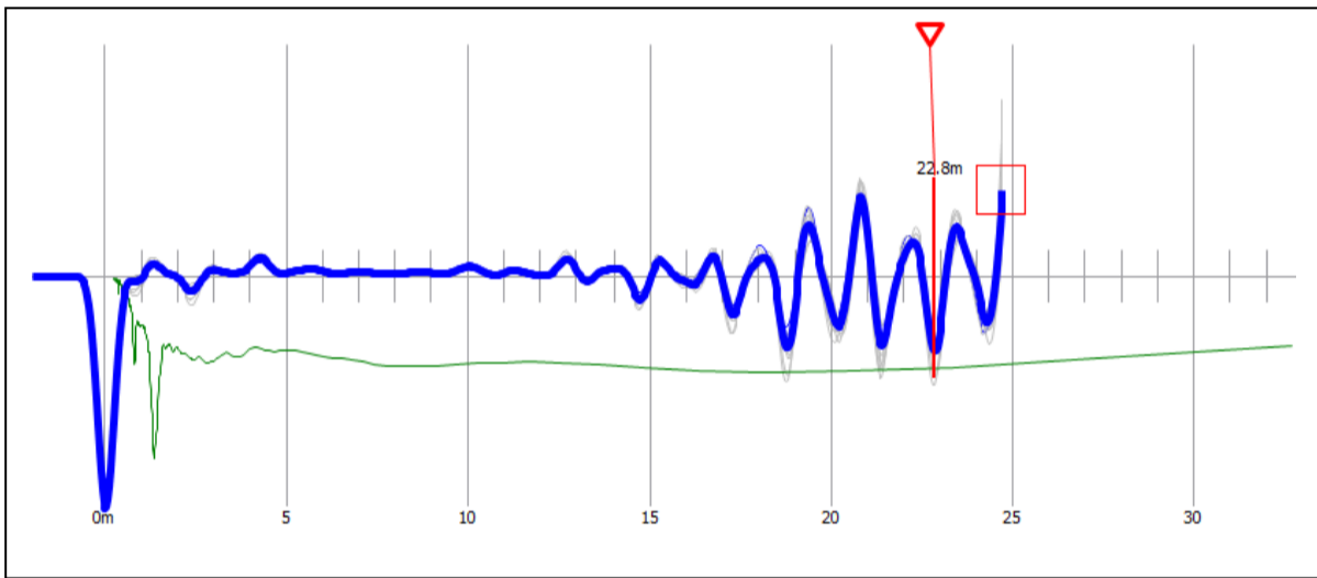
Reflectogram P-151
