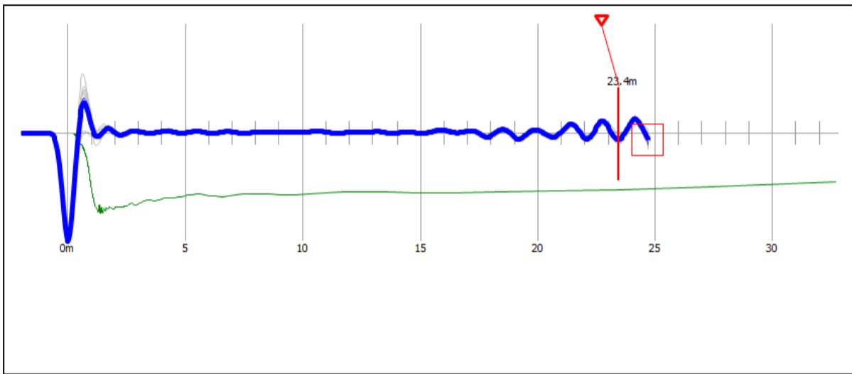
Reflectogram P-87
