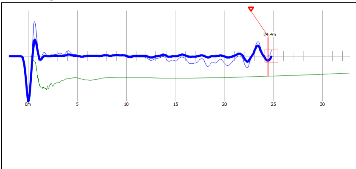
Reflectogram P-44
