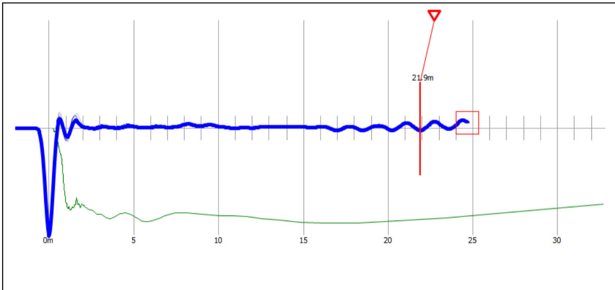
Reflectogram P-121
