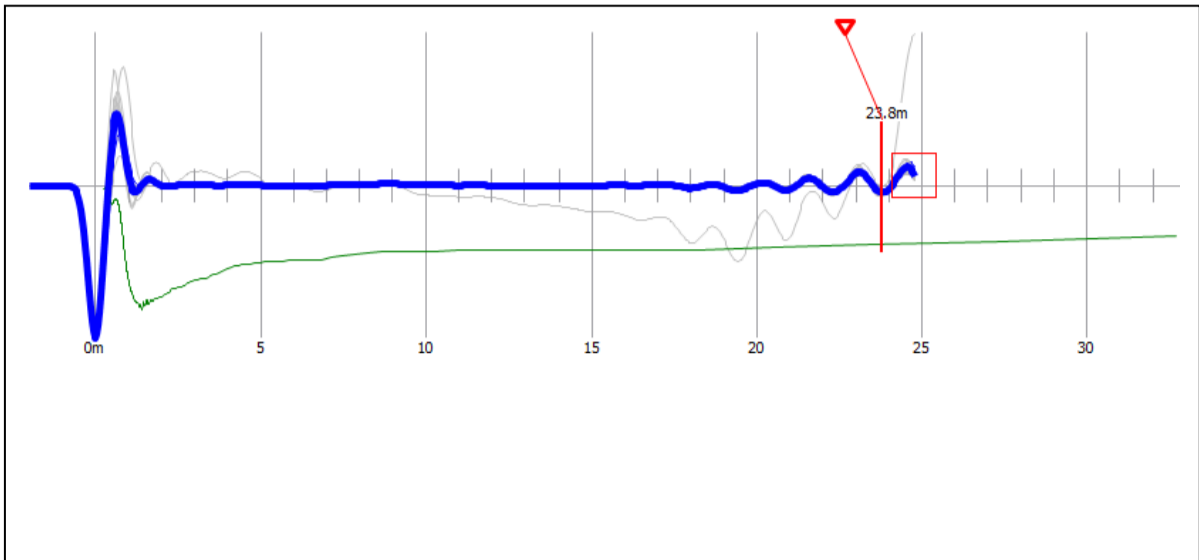
Reflectogram P-40
