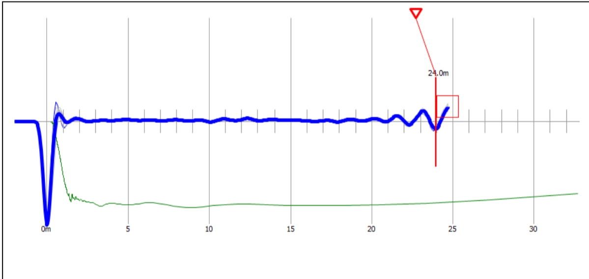
Reflectogram P-293
