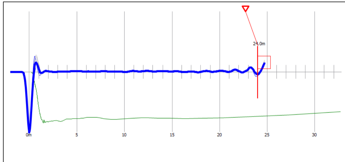
Reflectogram P-260
