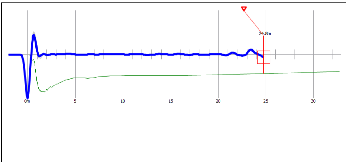
Reflectogram P-33
