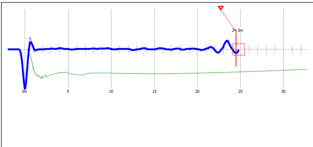
Reflectogram P-21
