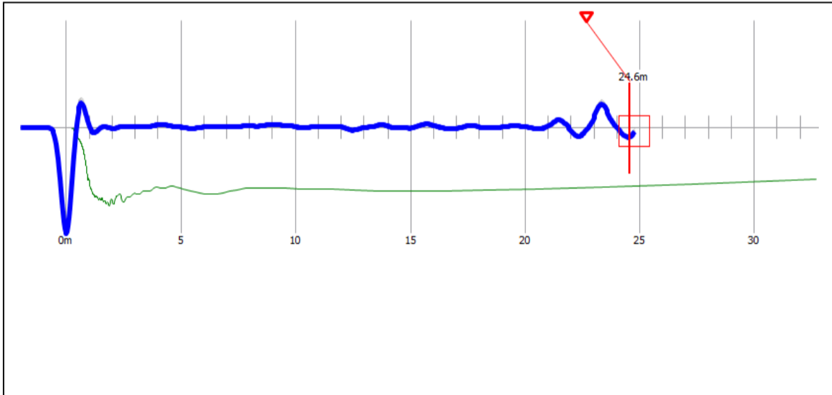
Reflectogram P-65
