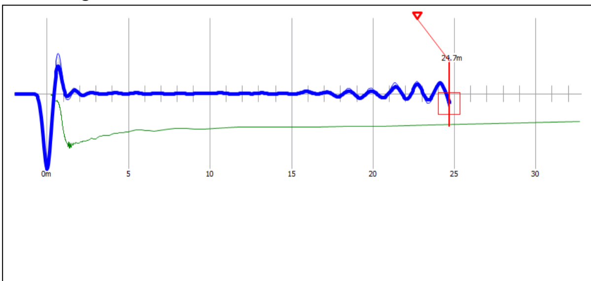
Reflectogram P-82
