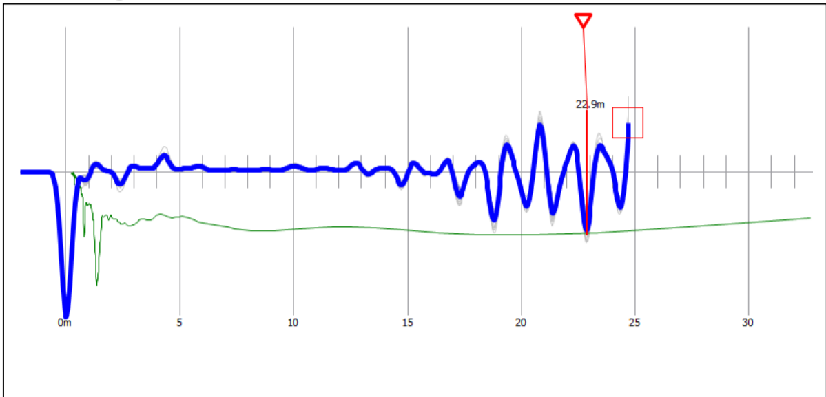
Reflectogram P-157
