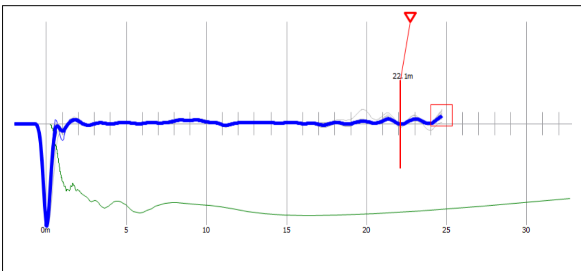
Reflectogram P-121
