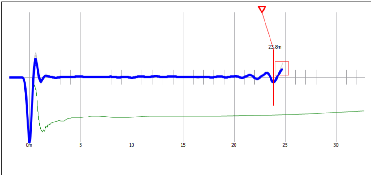
Reflectogram P-270
