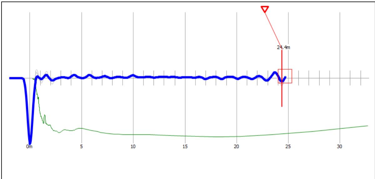
Reflectogram P-151
