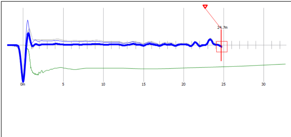
Reflectogram P-21
