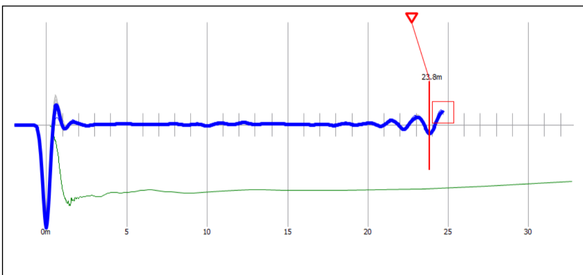
Reflectogram P-270
