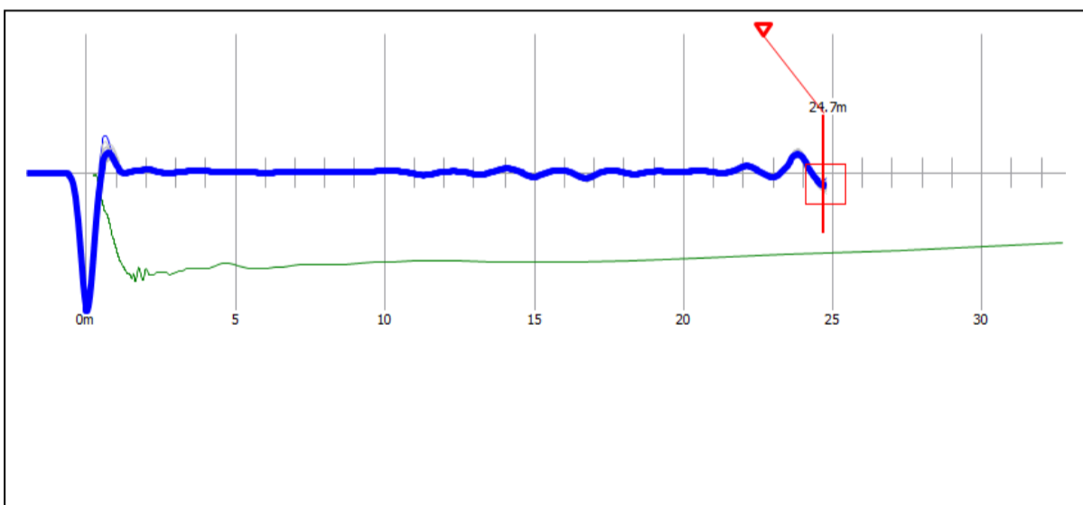
Reflectogram P-44
