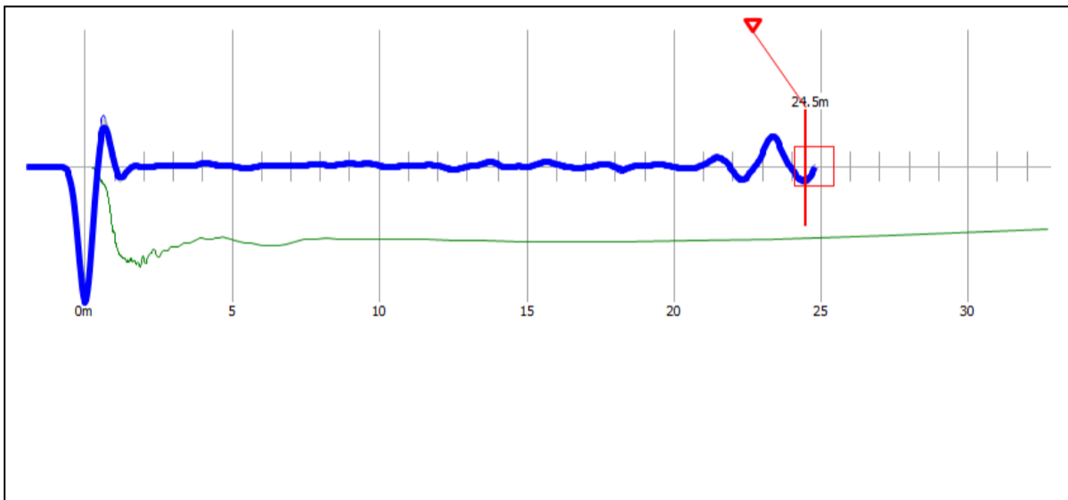
Reflectogram P-33
