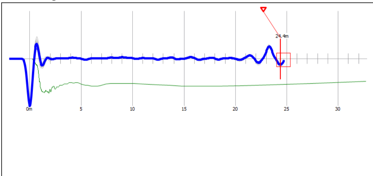
Reflectogram P-82
