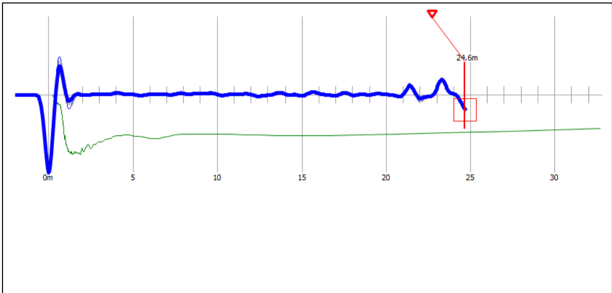
Reflectogram P-87
